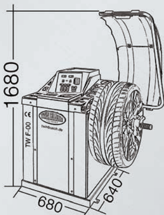
(1) Side holder for centering cones and gauge (2) Integrated distance measurement (3) Quick release nut \varnothing = 40 mm (4) 15 storage compartments (5) Digital Display (The new, compartment design ensures maximum user comfort and optimal ergonomics)
